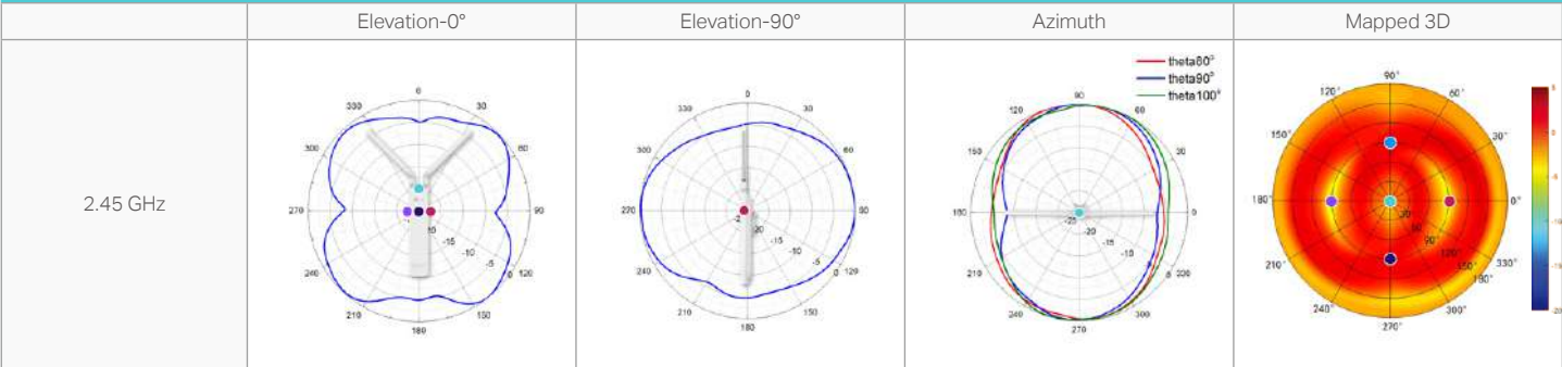
EAP110-Outdoor
