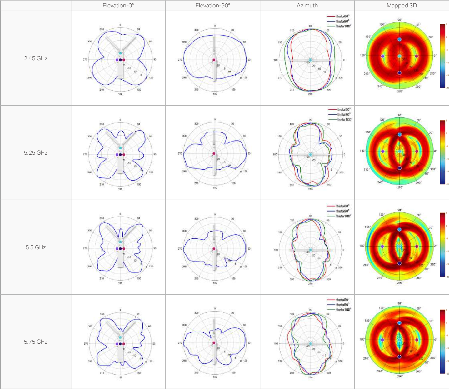
EAP225-Outdoor
